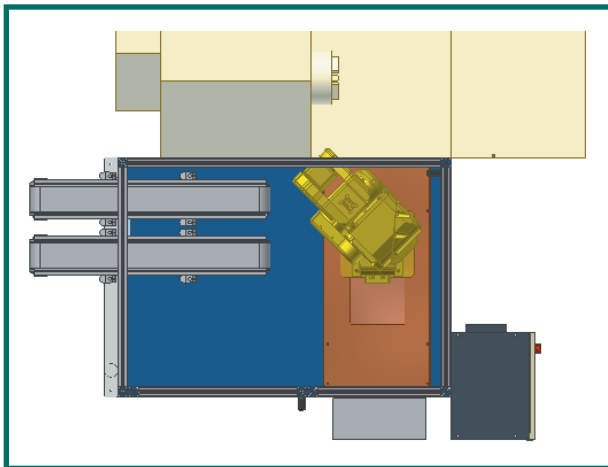
Lathe loader with powered infeed and exit conveyors
