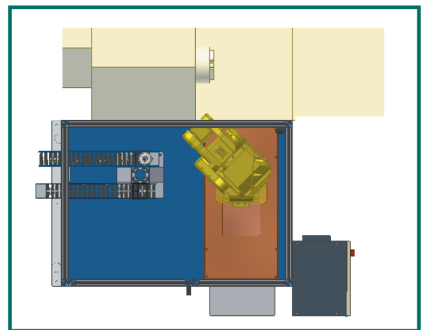
Lathe loader with gravity-powered infeed and exit conveyors
